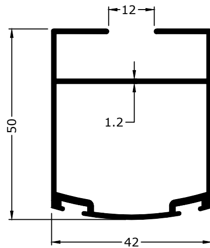
2018 0.727 KG/M
