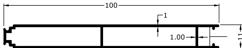
1717 0.625 KG/M
