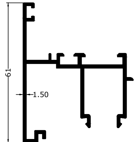
16961 0.870 KG/M
