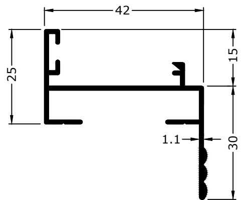
1018 0.410 KG/M
